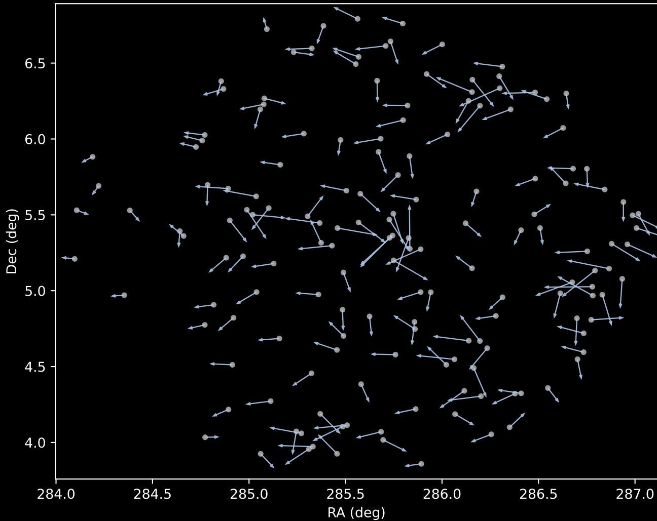
APOGEE DR17 Cluster 1 Proper Motion Vectors (n=160)
