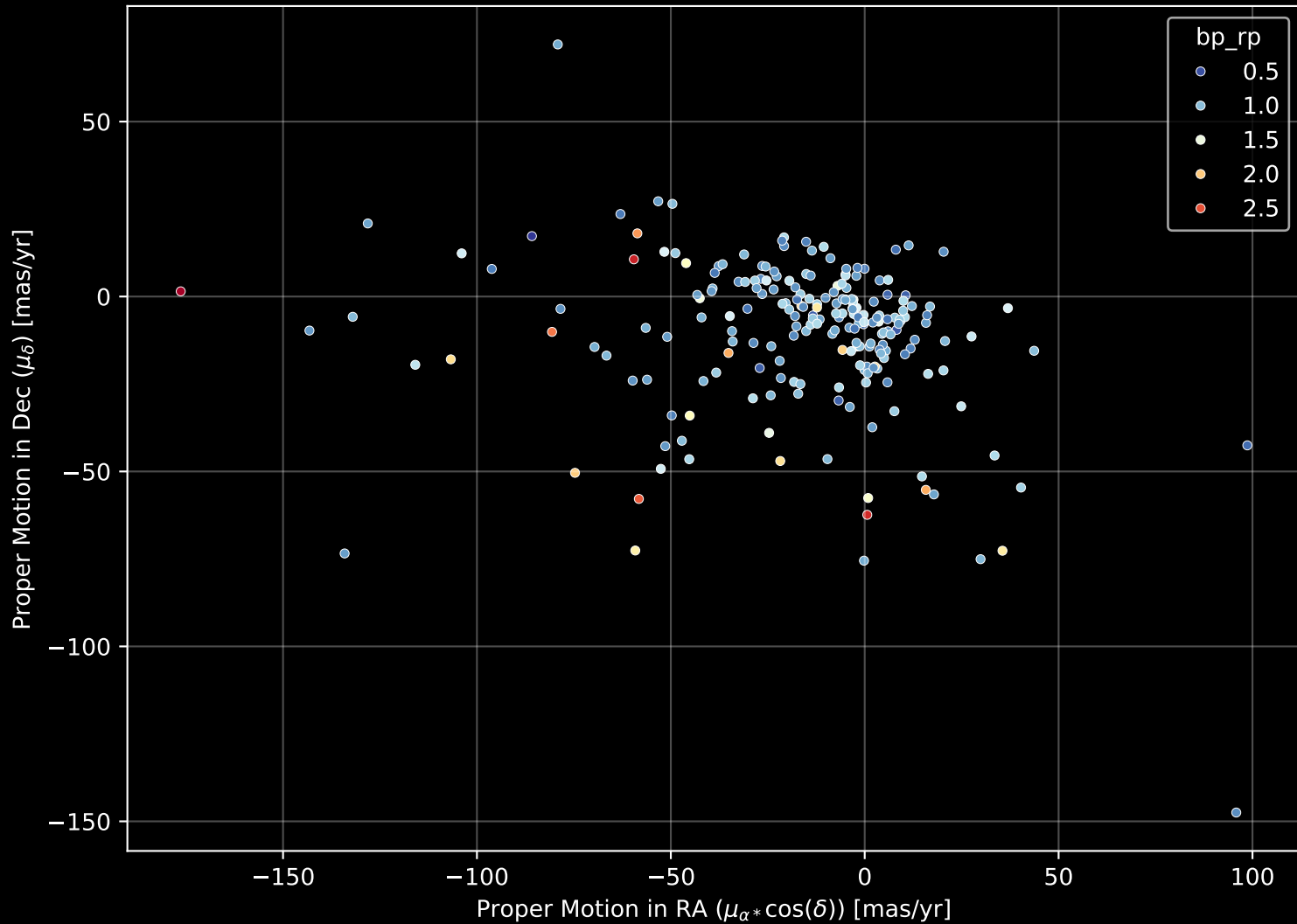
APOGEE DR17 Field: [283+67_btx] Proper Motion Diagram (n= 218)
