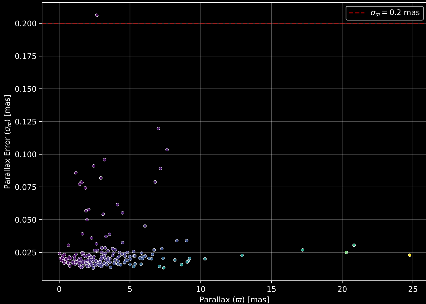
APOGEE DR17 Field: [283+67_btx] Parallax Quality (n= 218)
