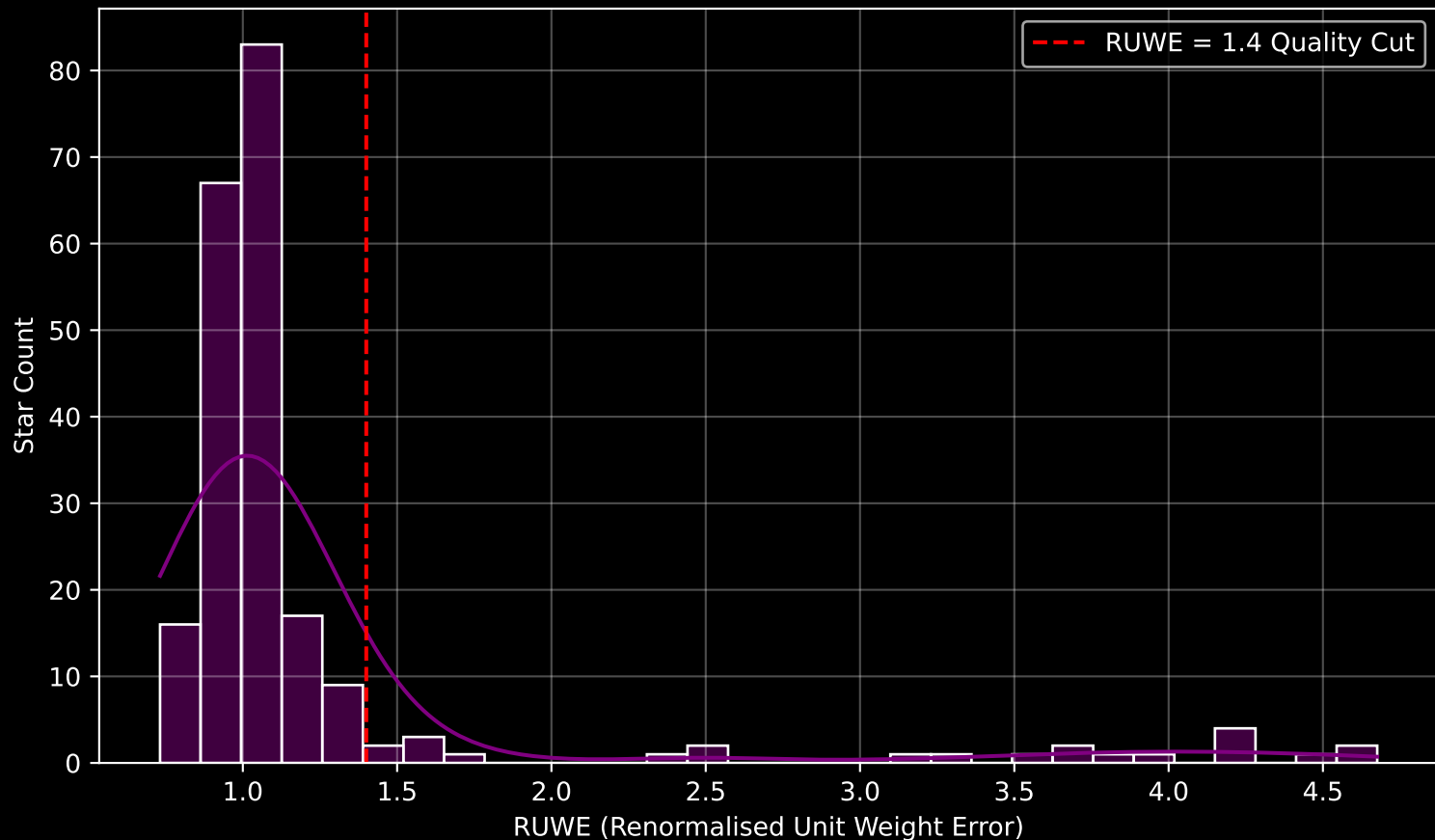
GAPOGEE DR17 Field [283+67_btx] RUWE Distribution (n= 215)
