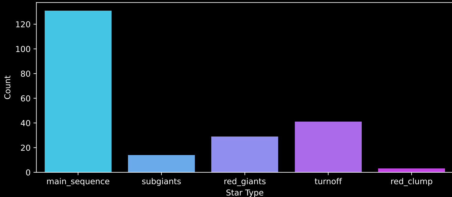
APOGEE DR17 Field: [283+67_btx] Count plot of Star Type
