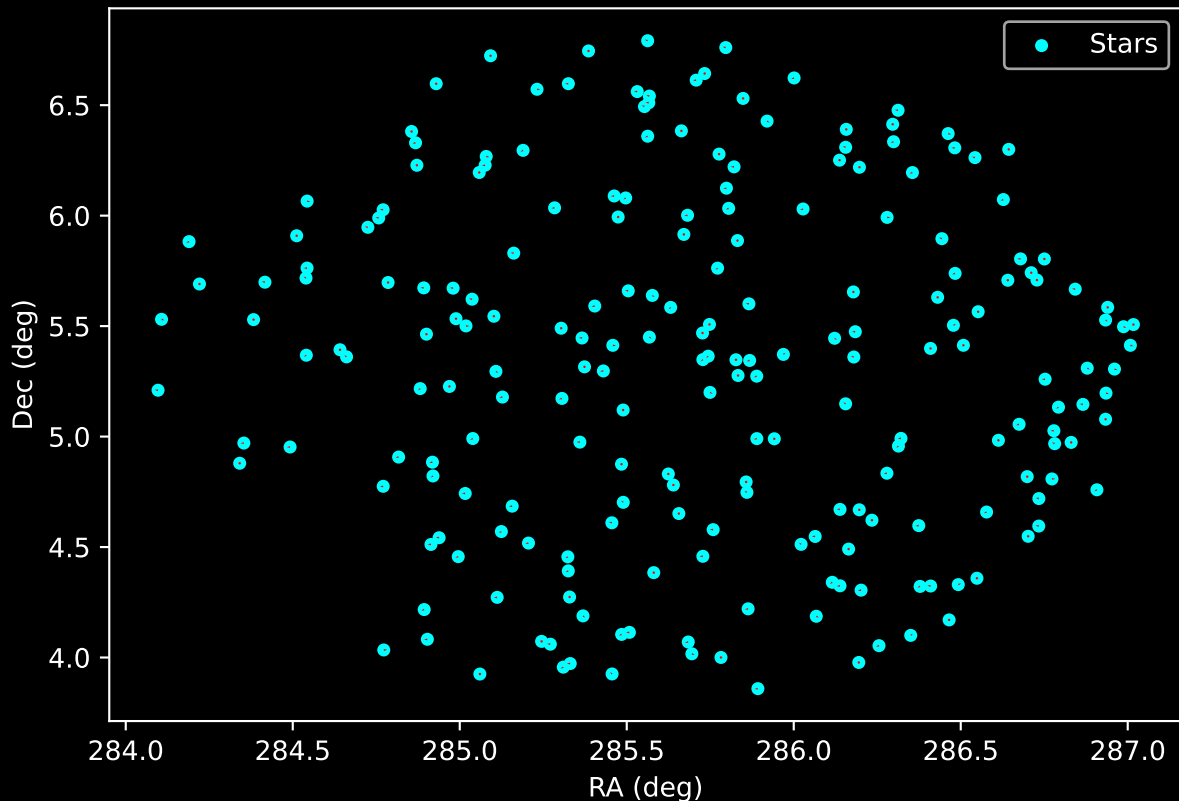
APOGEE DR17 Field: [283+67_btx] Proper Motion Vectors for Gaia Star Field (n= 218)
